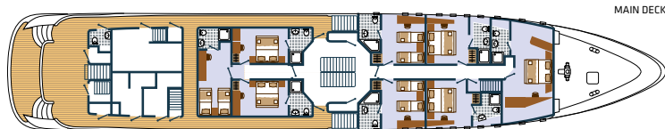
MAIN DECK
