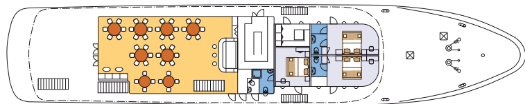
UPPER DECK
