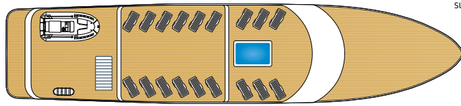
UPPER DECK
